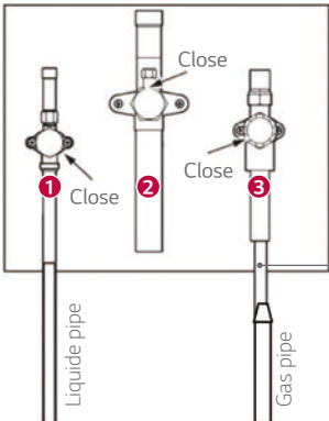
Heat Pump Installation
