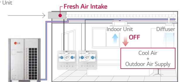
MULTI V 5 Outdoor unit
