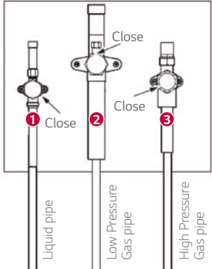
Heat Recovery Installation
